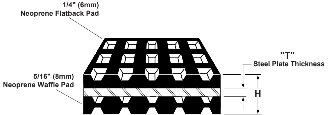
TYPE WMFB DIMENSIONS (inches)
