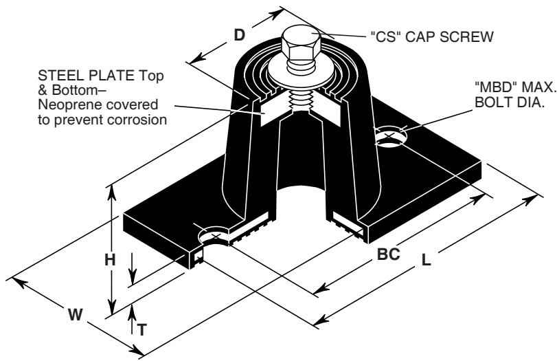
TYPE ND DIMENSIONS (mm)
