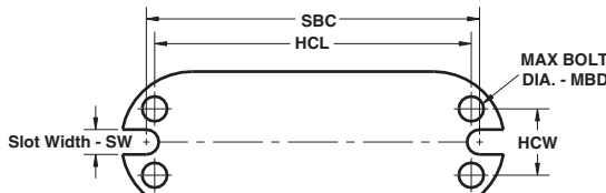
BASE PLATE DIMENSIONS
